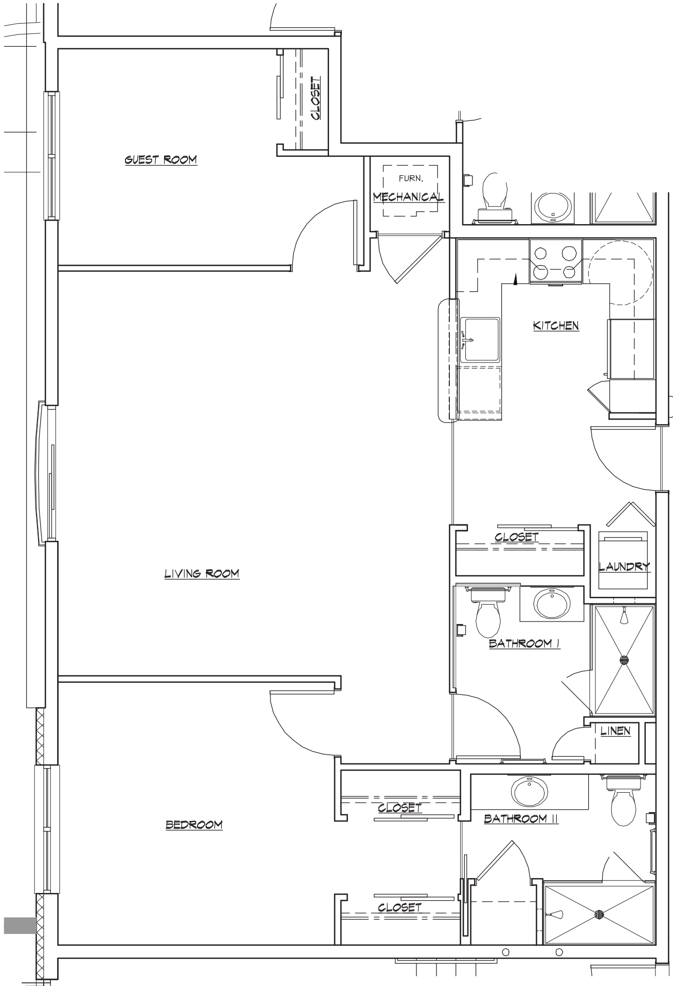
"TRIPHAMMER" Floor Plan: 1,110 square-feet; 2 Bedroom; 2 Bath
